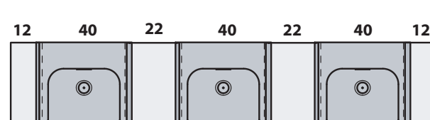
= 176 cm MODULO 3 LAVABI 40 / MODULE 3 WASHBASINS 40
