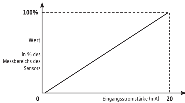
Sensorsignal 0–20 mA
