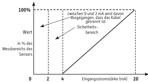
Sensorsignal 4–20 mA
