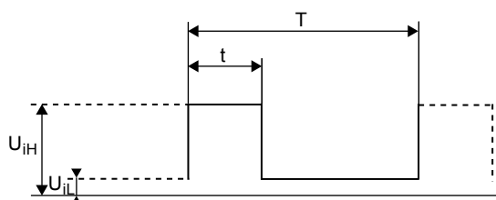
Fig. 49 Signal MLI
