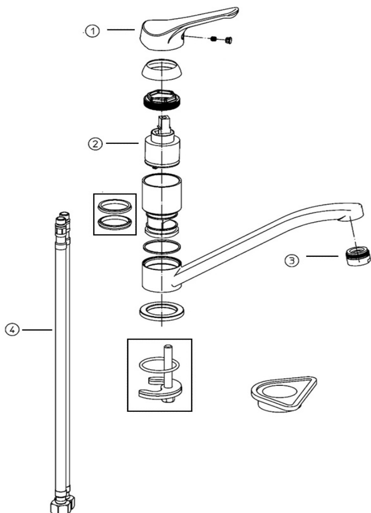
Tap Basic Spout Top HP CHR 115.0707.619
