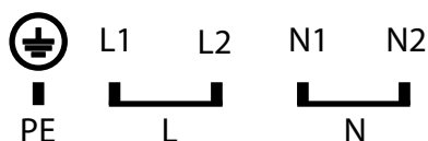
230 V ~, H05V2V2-F3×4,0
