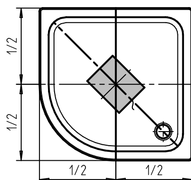
ZIRKON Mod. 507 800x1000 Mod. 509 1000x800 Mod. 510 1000x1000
