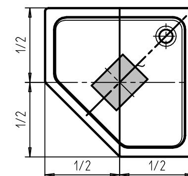
CORNEZZA Mod. 672 1000x1000 Mod. 673 1000x1000
