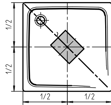
SUPERPLAN Mod. 391 1000x1000 Mod. 399 1200x1200
