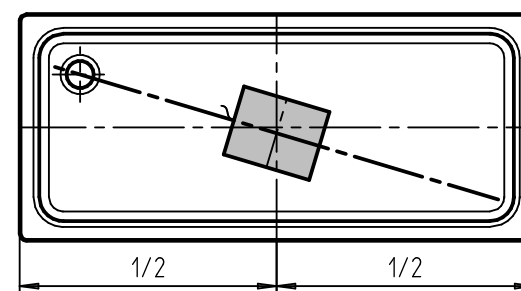
DUSCHPLAN Mod. 546 800x1000 Mod. 555 800x1200 Mod. 415 700x1200 Mod. 416 750x1000 Mod. 417 750x1200 Mod. 418 900x1000 Mod. 419 900x1100 Mod. 420 900x1200 Mod. 421 1000x1200
