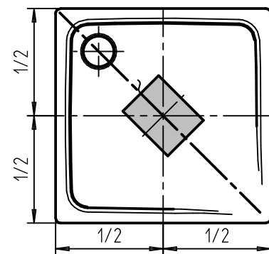
SUPERPLAN PLUS Mod. 479 1000x1000 Mod. 486 1200x1200
