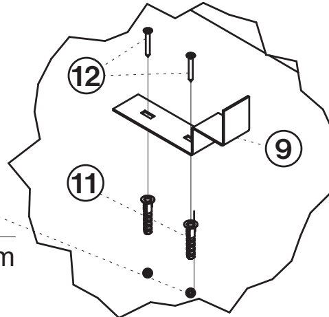
DETAIL E
