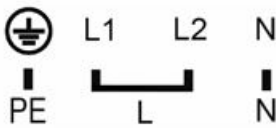
230 V ~, H05V2V2-F3x4,0 Fig. 3
