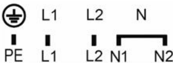
400 V 2N ~, H05V2V2-F4x4,0 Fig. 4
