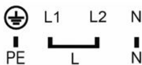
230 V ~, H05V2V2-F3x4,0
