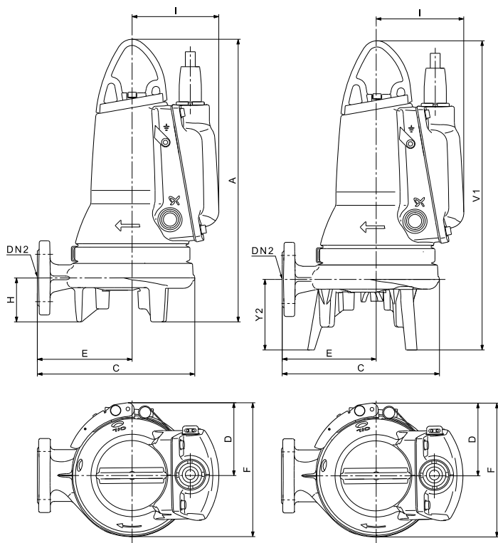
Fig. C Free-standing Installation
