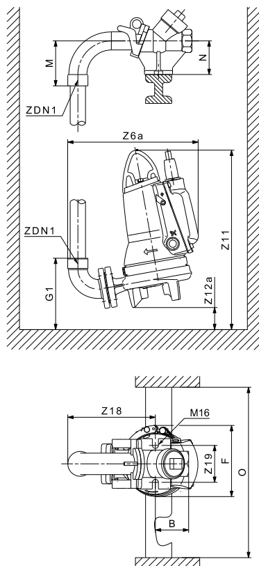
Fig. B One-pump installation on hookup auto-coupling
