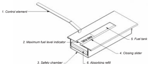
Picture 2. Bio-container – crossection
