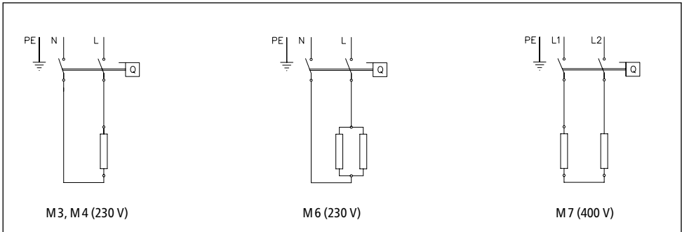
Afb. 8: "Schakelschema"
