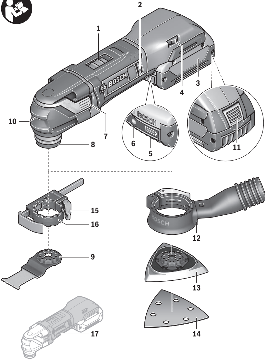
GOP 18V-28
