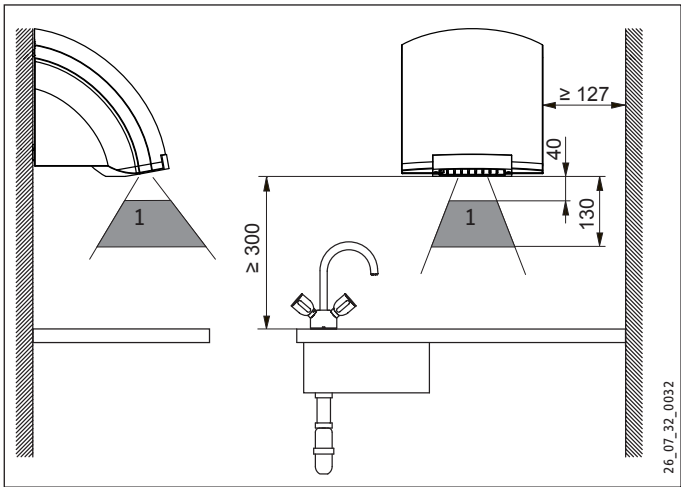
1 Detection range of IR proximity sensor
