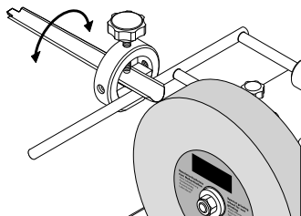
Device for tubes and gouges (with 100) 55, order no. 8949 0706
