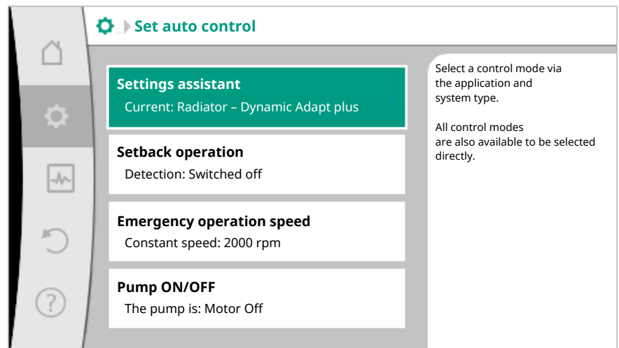
Fig. 49: Settings assistant
