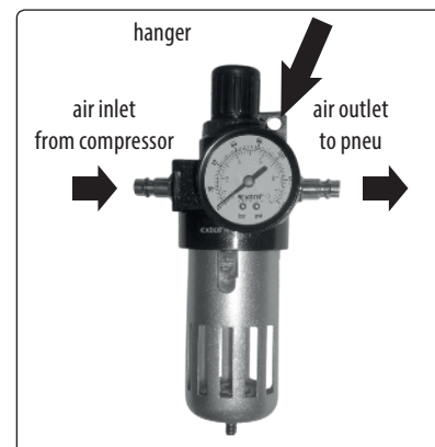
Fig. 7, description of the pressure regulator with pressure gauge and filter Extol® 8865104
