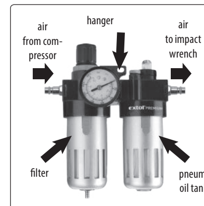
Fig. 8, description of the treatment unit Extol® 8865105
