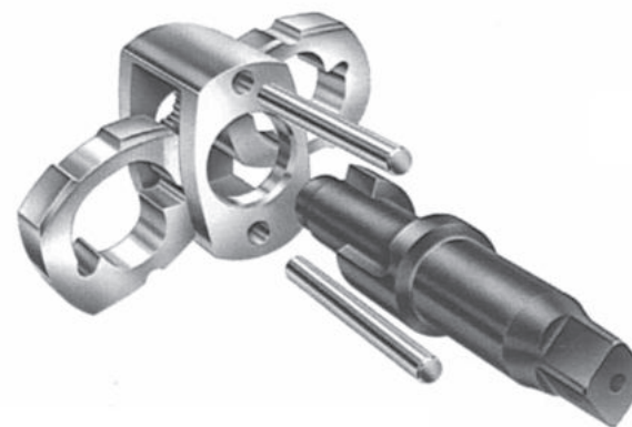
Obr. 1, systém Twin hammer
