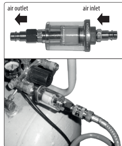
Fig. 6, filter connection (separator) Extol® Craft 8865101
