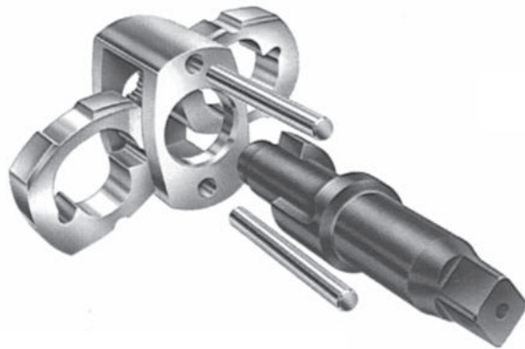
Abb. 1 System TWIN HAMMER
