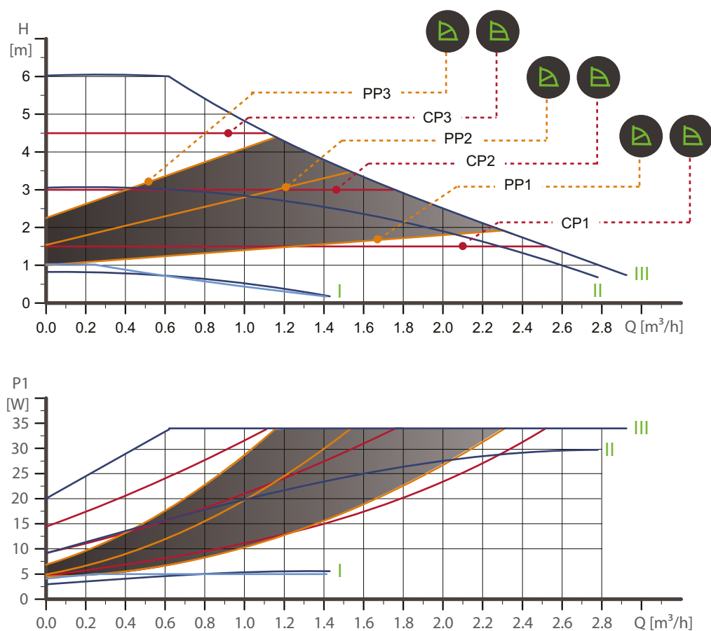
Obr. 41 ALPHA2 a ALPHA3, 25-60 A
