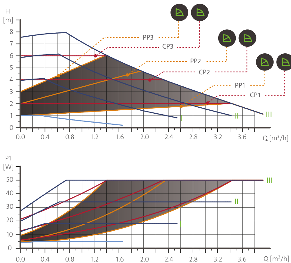
Obr. 42 ALPHA2 a ALPHA3, 25-60 A
