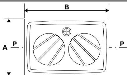
GIGANT PRO 80x100 A = 800, B = 1000 GIGANT PRO 80x110 A = 800, B = 1100 GIGANT PRO 80x120 A = 800, B = 1200 GIGANT PRO 90x120 A = 900, B = 1200
